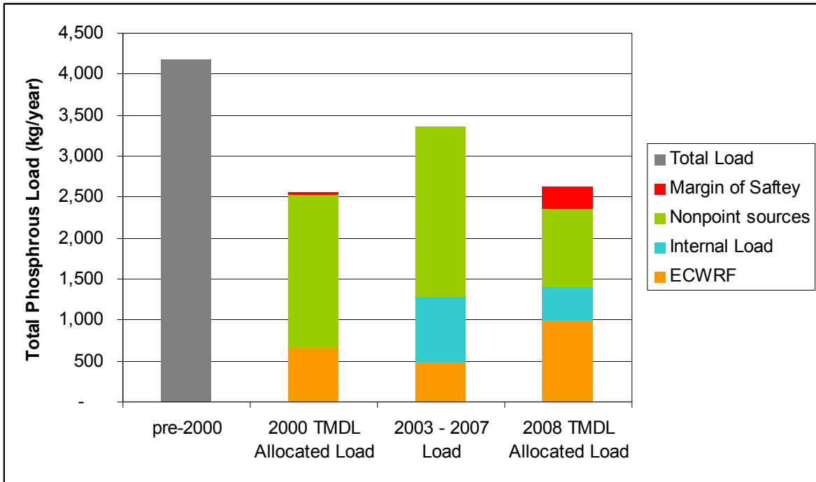
Figure 7.3. Change in total phosphorus load and allocations for the East Canyon Reservoir TMDL.
